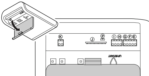
Fig. 7: Opening the drive head cover
